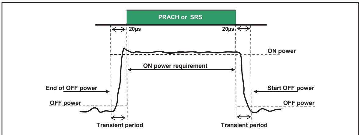
Figure 6.3.4.2-1: PRACH and SRS ON/OFF time mask
