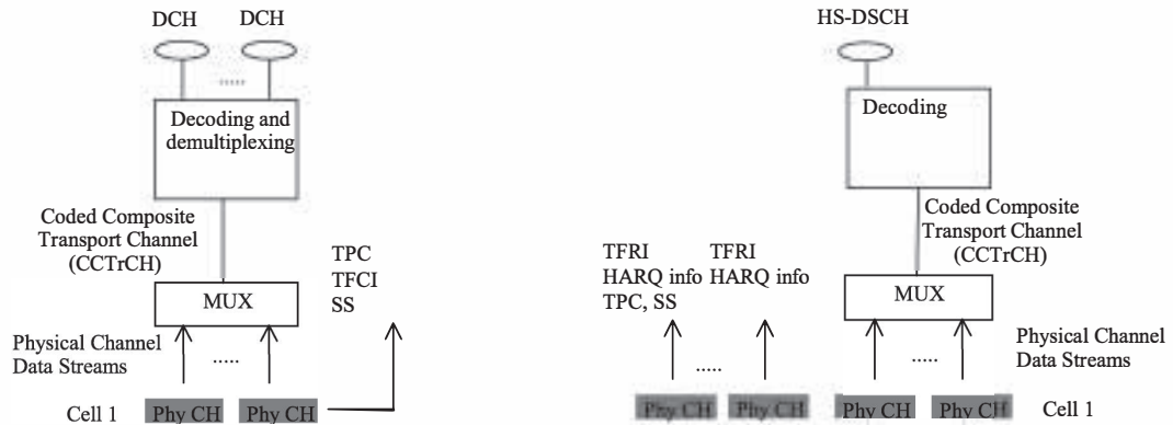
DCH model with HS-DSCH(s)
