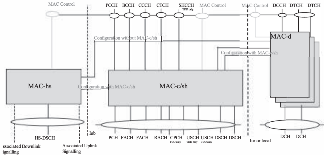
Figure 6.2.1-1: UTRAN side overall MAC architecture
