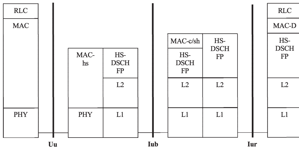
Figure 5.1-1: Protocol Architecture of HS-DSCH, Configuration with MAC-c/sh
