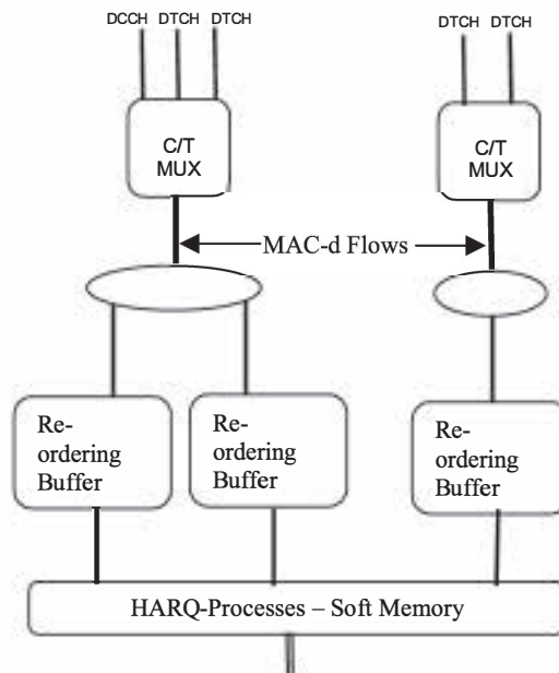
Figure 6.1.2-1: MAC-d architecture
