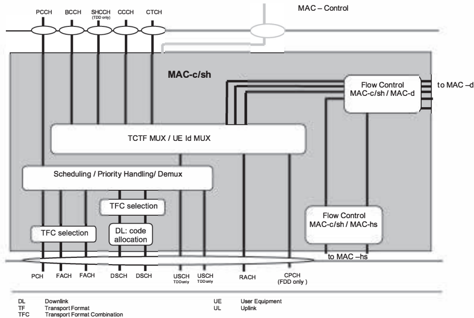
Figure 6.2.2-1: UTRAN side MAC architecture/MAC-c/sh details
