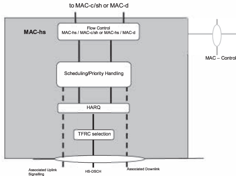
Figure 6.2.3-1: UTRAN side MAC architecture/MAC-hs details
