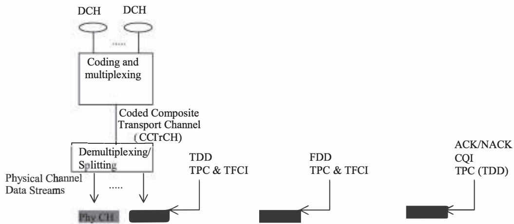
Figure 5.2.3-1: Model of the UE's Uplink physical layer
