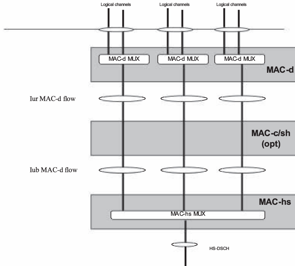
Figure 6.2.1-2: UTRAN side of MAC multiplexing
