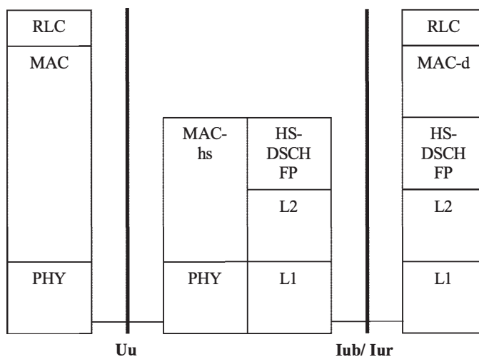
Figure 5.1-2: Protocol Architecture of HS-DSCH, Configuration without MAC-c/sh
