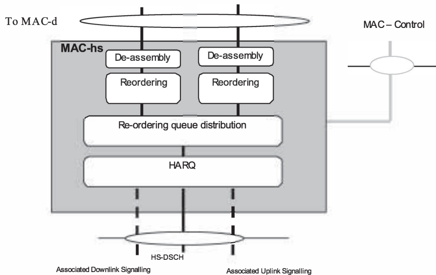
Figure 6.1.4-1: UE side MAC architecture/MAC-hs details
