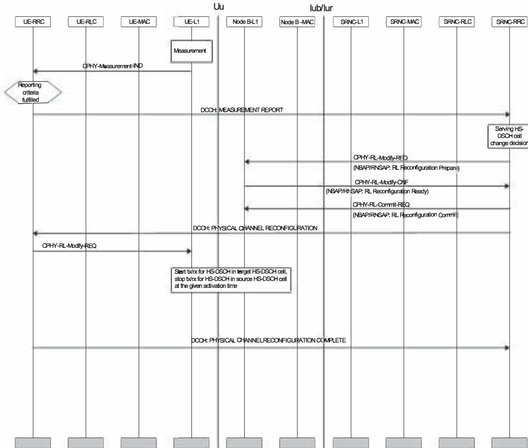
Figure 9.3-1: Intra-Node B synchronised serving HS-DSCH cell change
