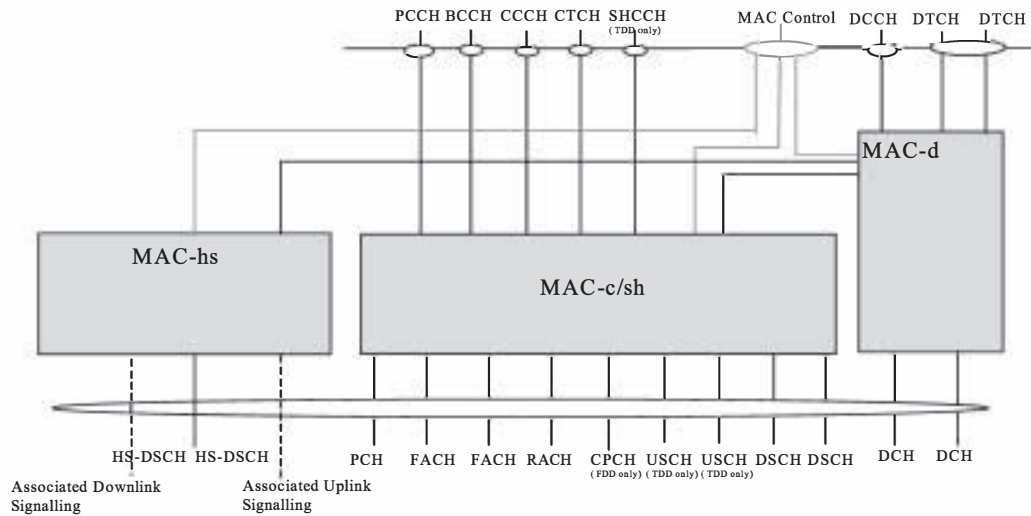
Figure 6.1.1-1: UE side MAC architecture with HS-DSCH
