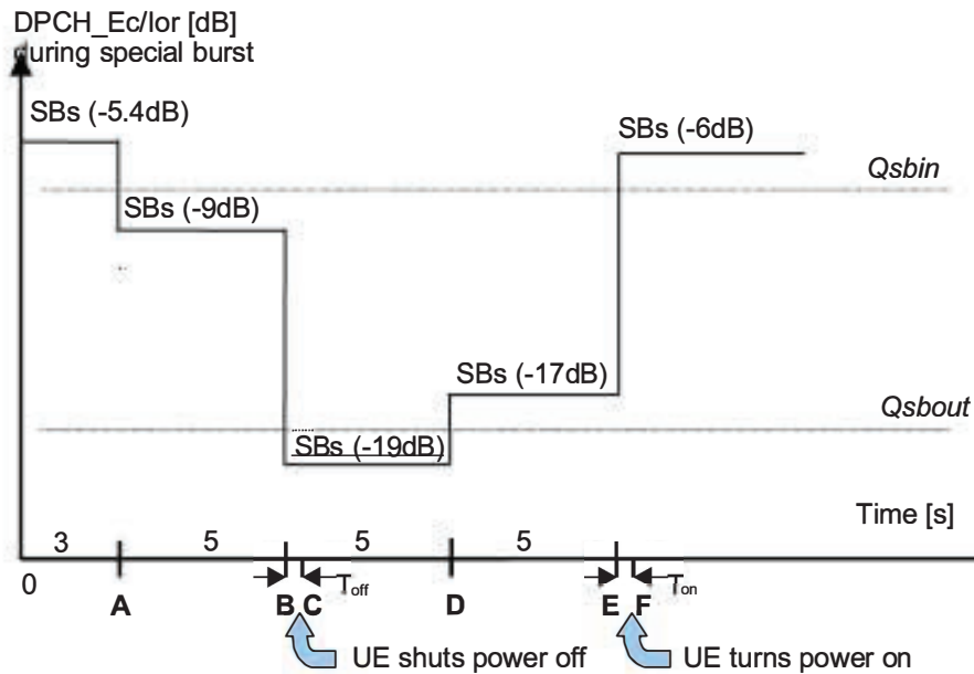
Figure 6.1B: Test case for out-of-synch handling in the UE -1.28 Mcps TDD option - discontinuous transmission
