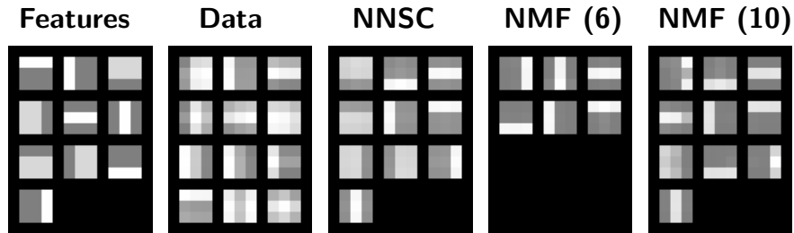
Figure 1: Experiments on bars data. Features: The 10 original features that were used to construct the dataset. Data: A random sample of 12 data vectors. These constitute superpositions of the original features. NNSC: Features learned by NNSC, with dimensionality of the hidden representation equal to 10, starting from random initial values. NMF (6): Features learned by NMF, with dimensionality 6. NMF (10): Features learned by NMF, with dimensionality 10. See main text for discussion.
