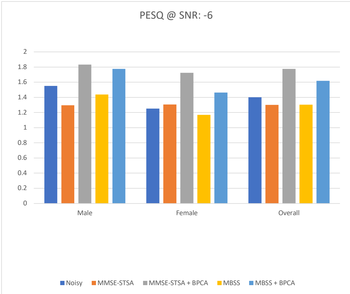
Figure 4.1.2: Average PESQ scores in -6 dB SNR for male and female speakers under ‘Babble’ noise contamination [80].
