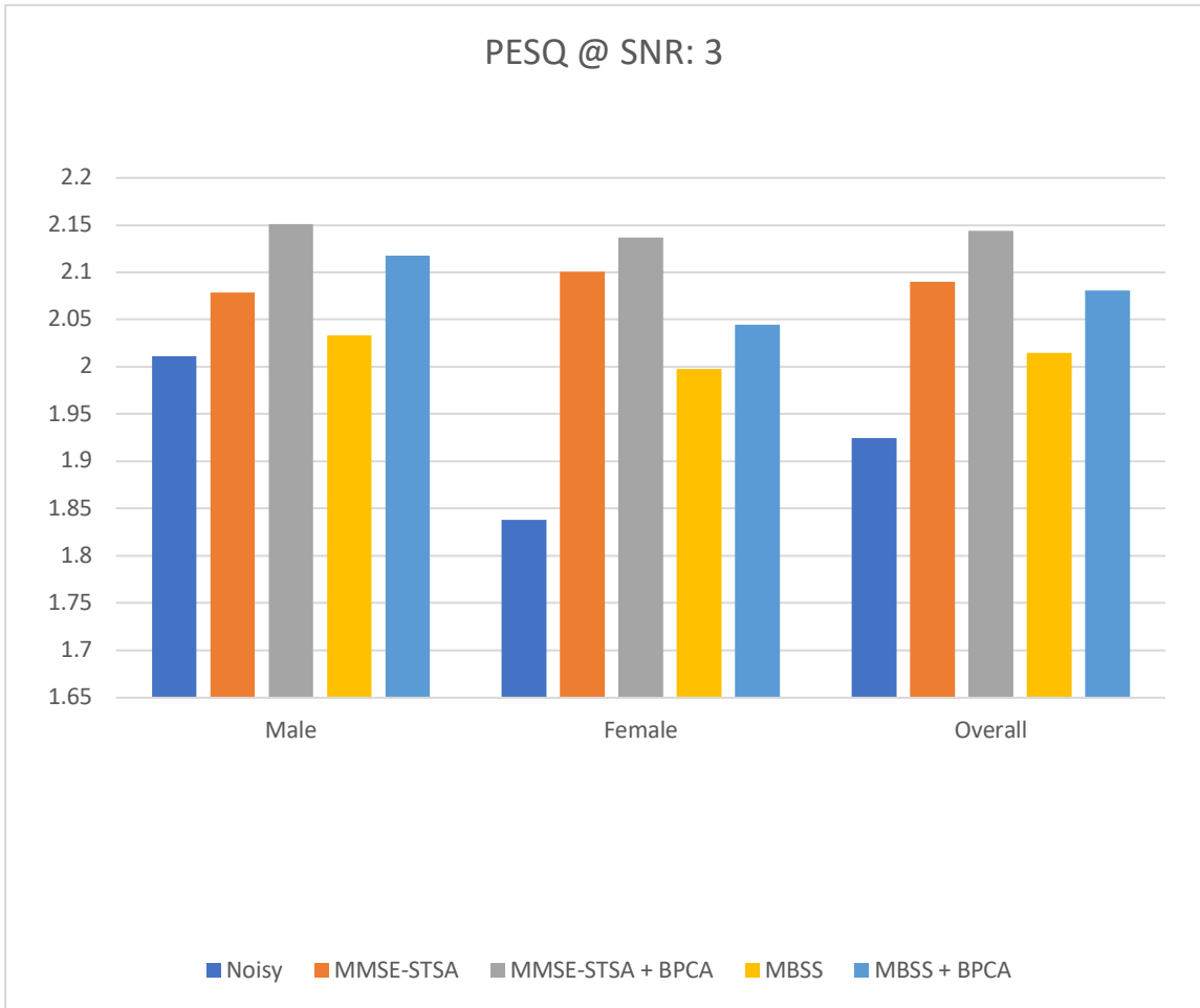
Figure 4.1.5: Average PESQ scores in 3 dB SNR for male and female speakers under 'Babble' noise contamination [80].
