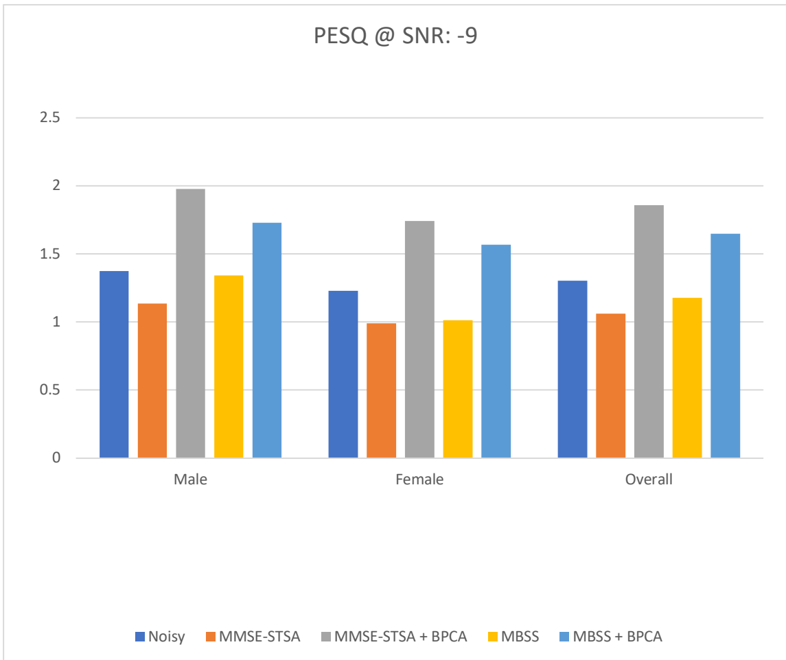
Figure 4.1.1: Average PESQ scores in -9 dB SNR for male and female speakers under 'Babble' noise contamination [80].
