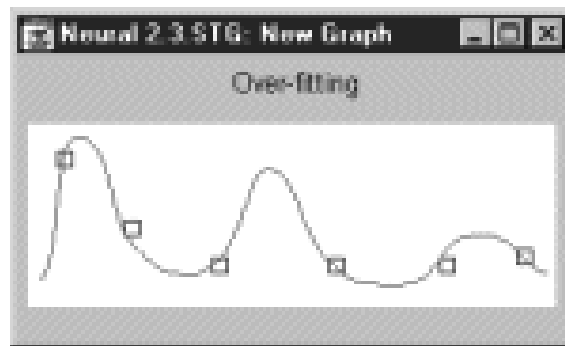
Fig. 4. High-order polynomial sample
