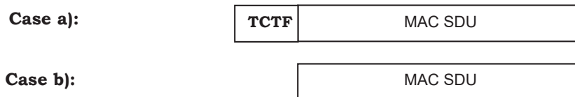
Figure 9.2.1.6.1: MAC PDU format for SHCCH
