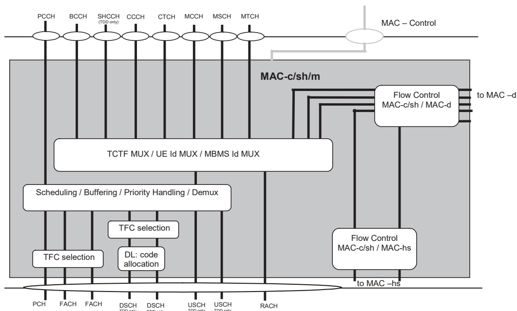
Figure 4.2.4.1.1: UTRAN side MAC architecture / MAC-c/sh/m details
