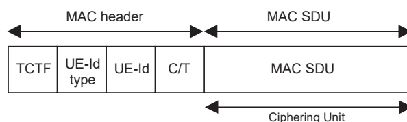
Figure 11.5.1: Cipherrered part unit for a MAC PDU
