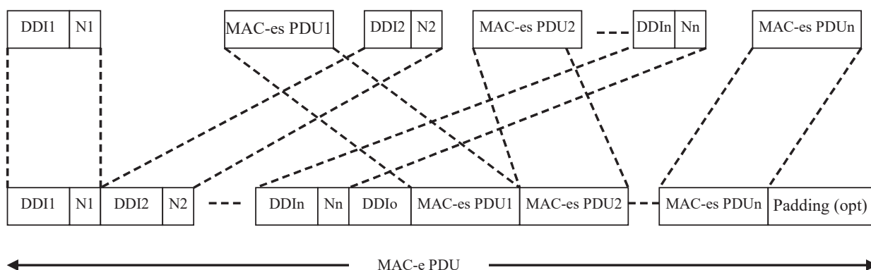
Figure 9.1.5.2: MAC-e PDU
