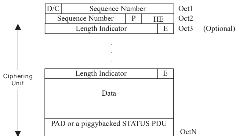
Figure 9.20: Cipherng unit for an AMD PDU
