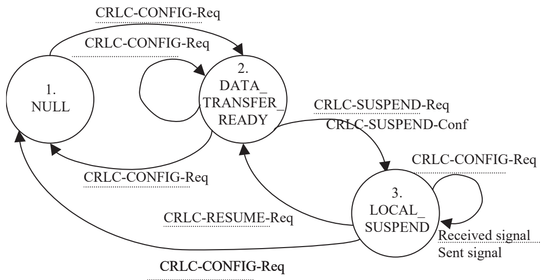
Figure 9.17: The state model for unacknowledged mode entities
