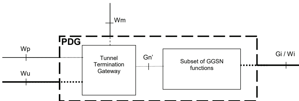
Figure F.1: PDG implementation re-using GGSN functionality
