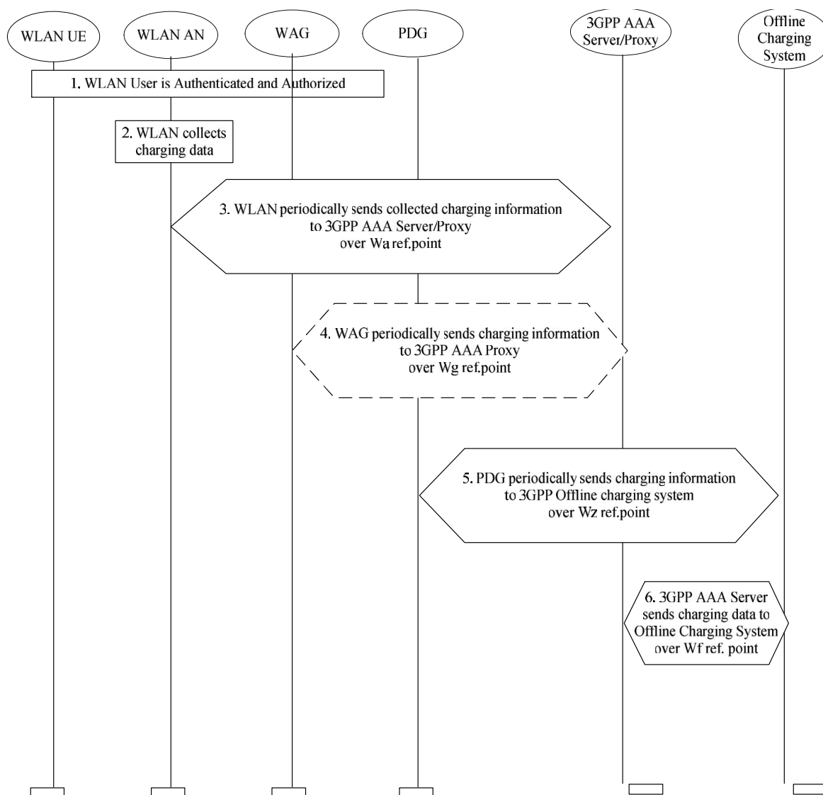
Figure 7.8: Charging Procedure for Offline Charged Subscribers
