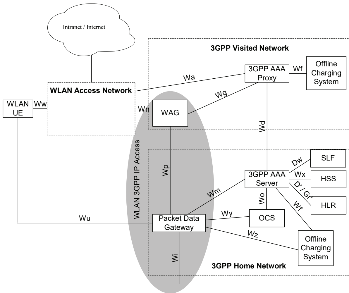
Figure 6.2a: Roaming reference model - 3GPP PS based services provided via the 3GPP Home Network
