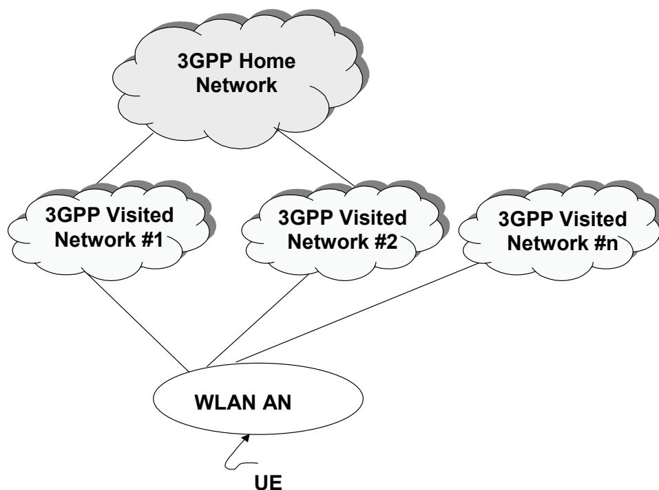
Figure 5.1: Network Advertising and Selection Scenario
