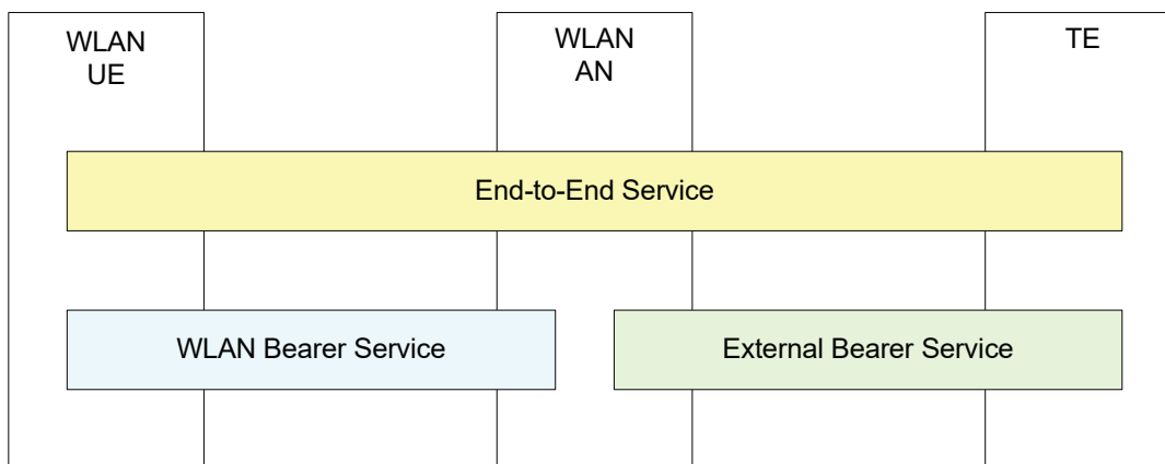
Figure 5.3: QoS Architecture for WLAN Direct IP Access
