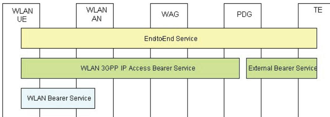
Figure 5.4: QoS Architecture for WLAN 3GPP IP Access
