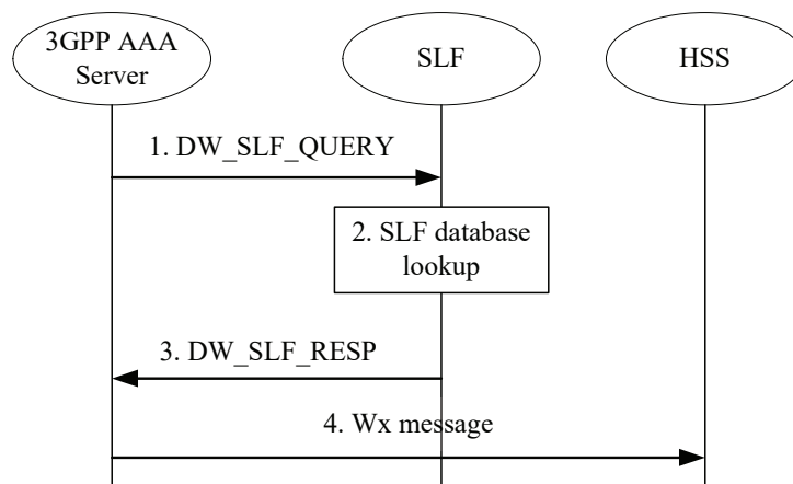
Figure 7.14: Query through SLF
