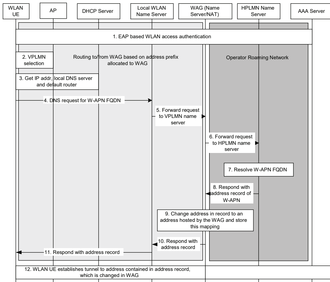
Figure C.2.2: DNS controlled reverse NAT procedure
