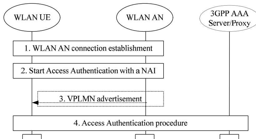
Figure 7.1: I-WLAN and VPLMN selection procedure
