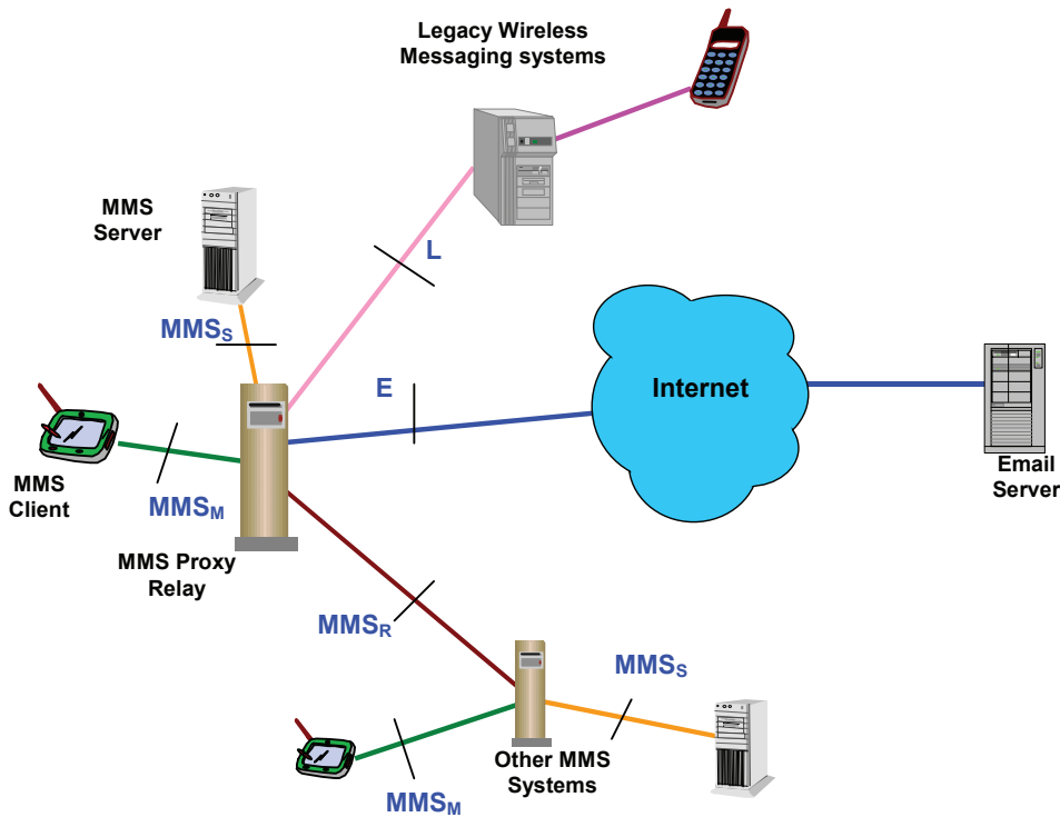
Figure 2 MMS Network Representation
