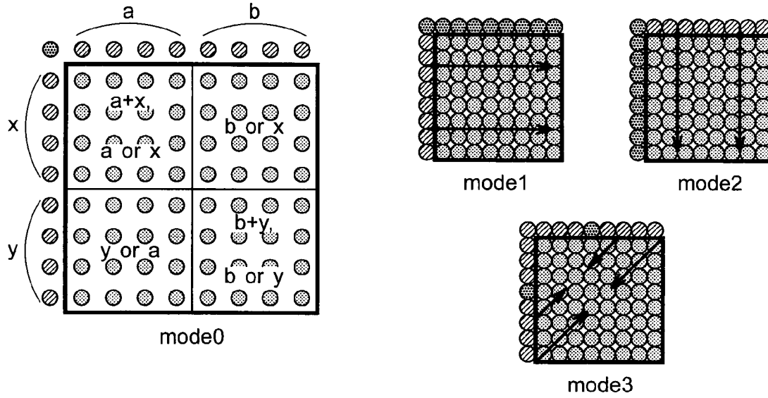
4:2:0/4:2:2 Cb/Cr INTRA PREDICTION
