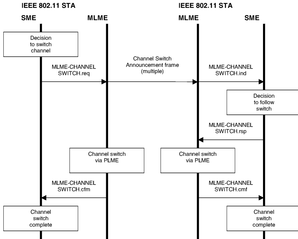
Figure 67e—Channel switch
