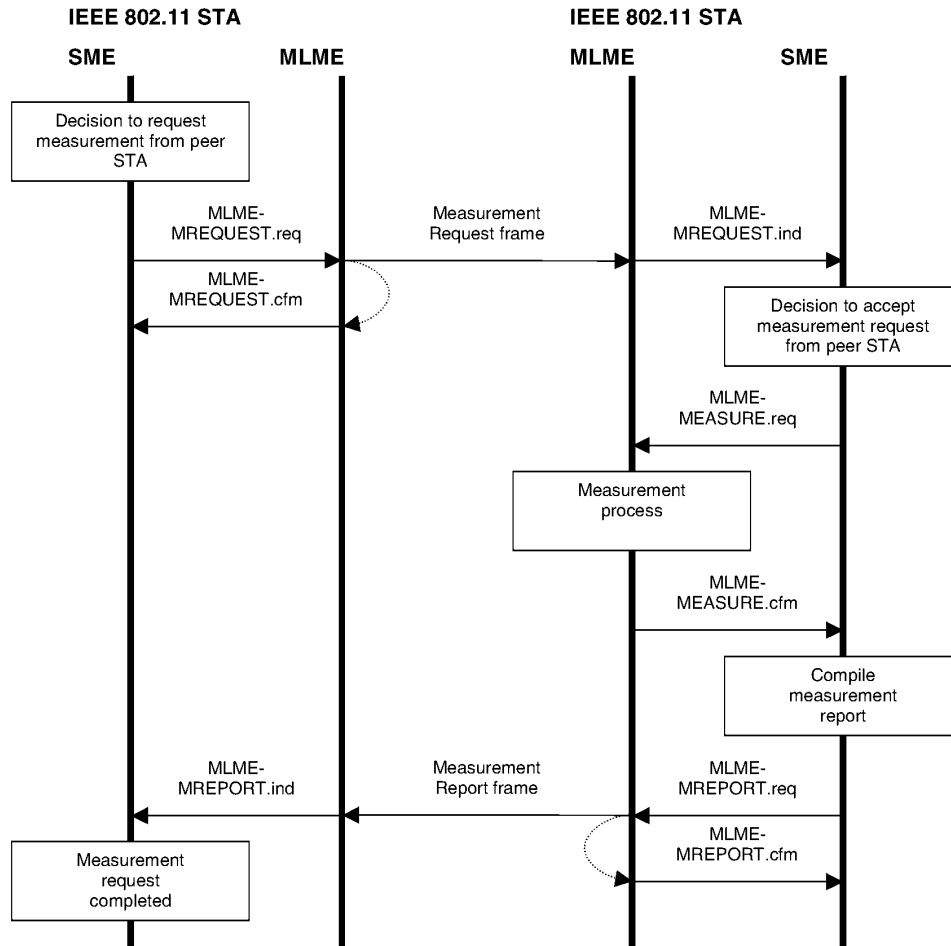
Figure 67b—Measurement request—accepted
