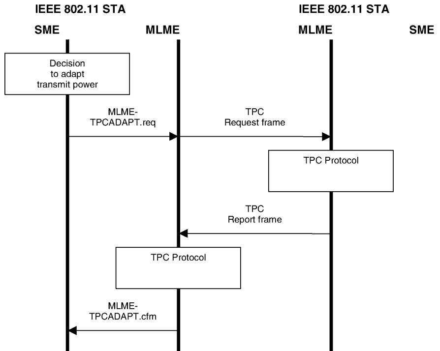
Figure 67d—TPC adaptation
