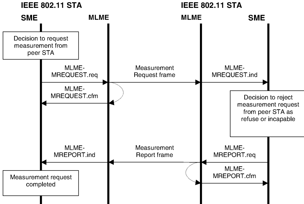
Figure 67c—Measurement request - rejected
