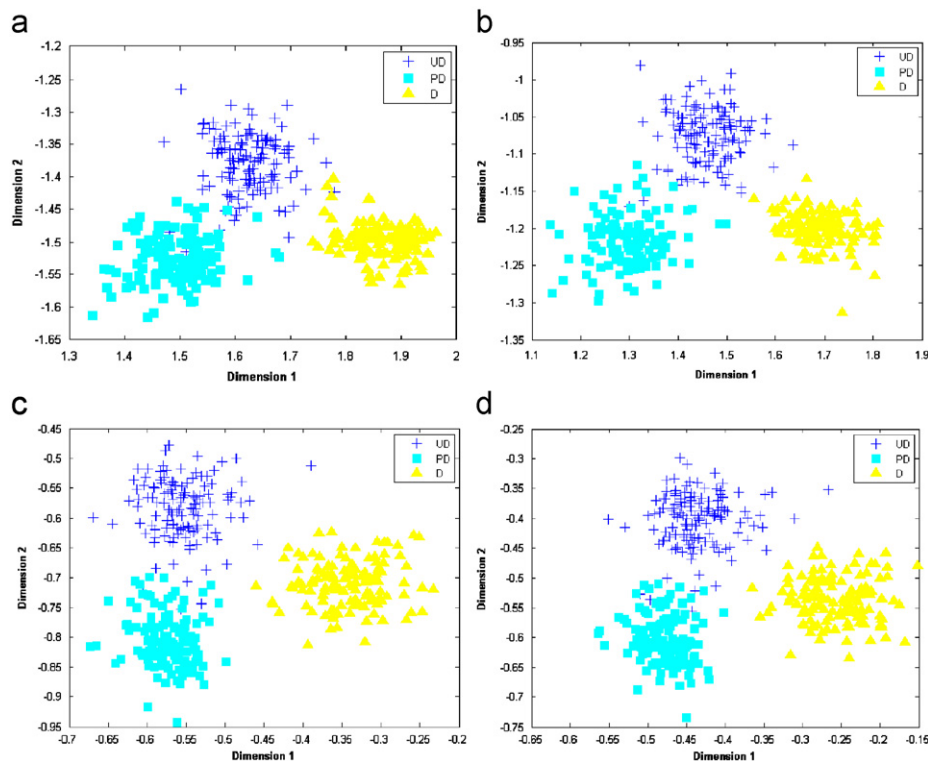
Fig. 7. Scatter plots of the training features in a two-dimensional feature space associated with four resolution levels (from the lowest to highest) are shown in (a)–(d). These features are selected and extracted when LDA and the classifier of KNN ( K = 5 ) are used.
