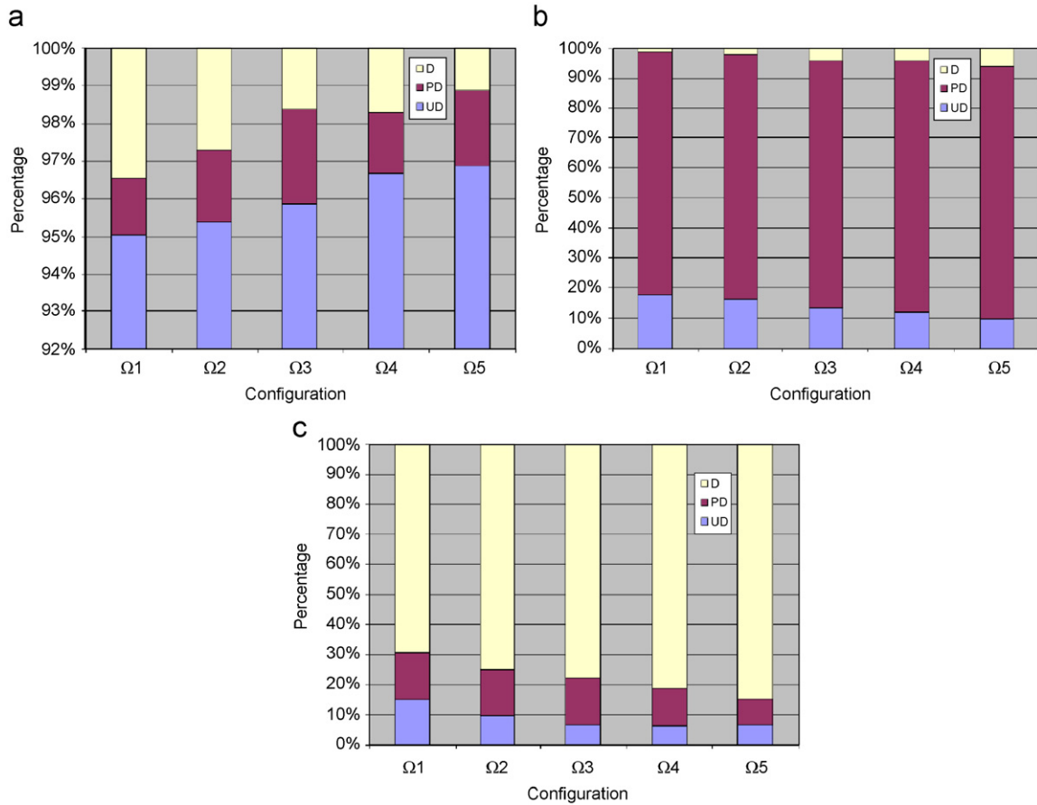
Fig. 8. Percentages of image tiles graded as undifferentiated, poorly differentiated, and differentiating for the three testing slides (i.e., Nos. 1–3 in Table 6) are shown in (a)–(c), respectively. For each slide, classification results associated with confidence configurations \Omega_1 – \Omega_5 in Table 7 are presented, respectively. For better visual effects, the vertical axis of (a) starts with 92%.
