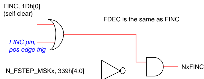
Figure 56. Logic Diagram of the FINC/FDEC Masks
