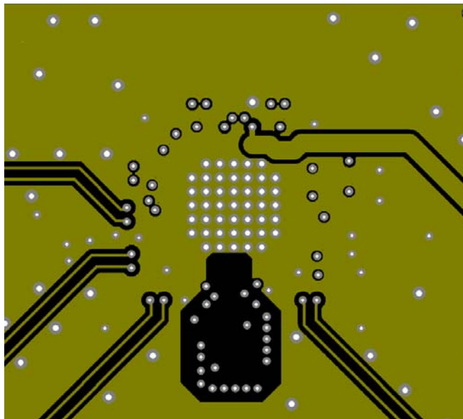
Figure 52. Clock Input Traces (Layer 5)
