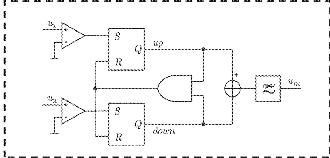
Phase Detector 2206''
