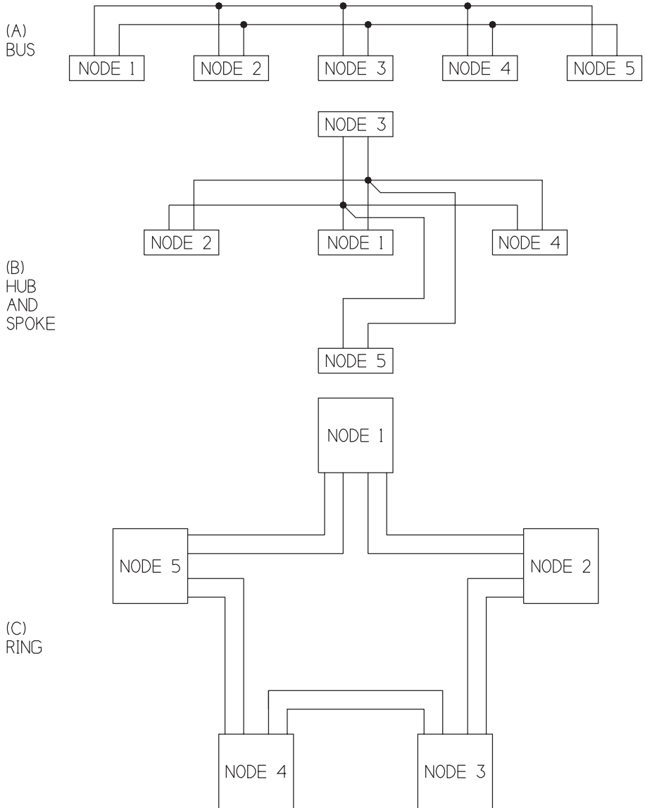
Figure 7-9: Network nodes can connect using any of several wiring topologies.
