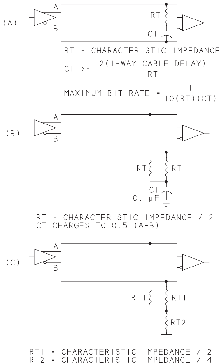
Figure 7-8: These terminations can conserve power on some lines.
