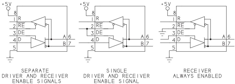
Figure 6-13: Three options for controlling the driver-enable and receiver-enable inputs on an RS-485 transceiver.
