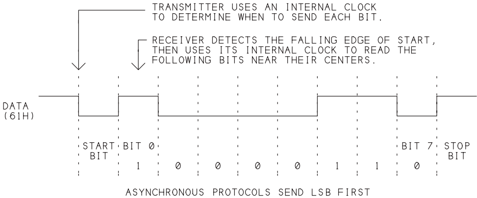
Figure 2-1: Synchronous transmissions include a clock line, while asynchronous transmissions require each computer to have its own clock.
