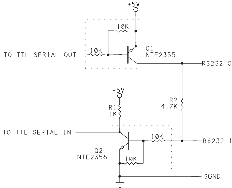
Figure 4-4: This half-duplex interface uses the RS-232 input's negative voltage to pull the RS-232 output below ground.
