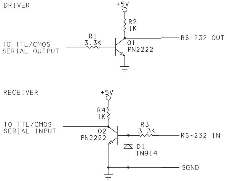
Figure 4-3: This 5V-only interface will work on many short links.
