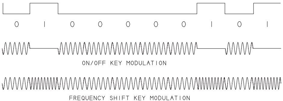
Figure 8-1: Wireless data often uses OOK or FSK modulation.
