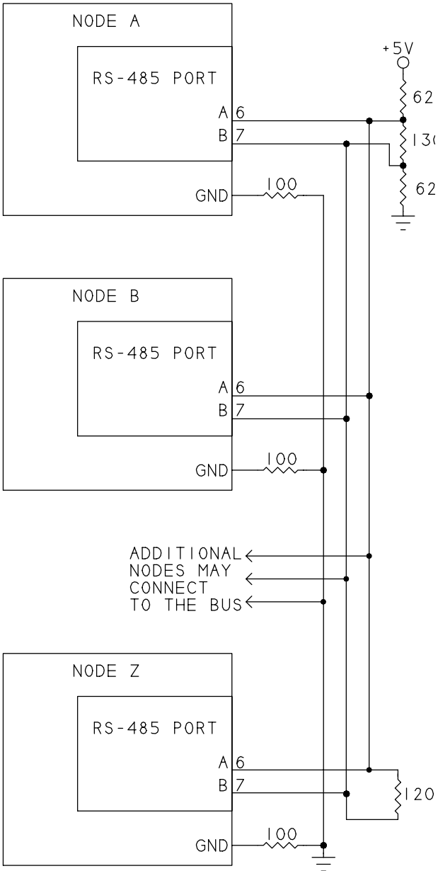
Figure 13-1: The RS-485 network can use this wiring to connect the r
