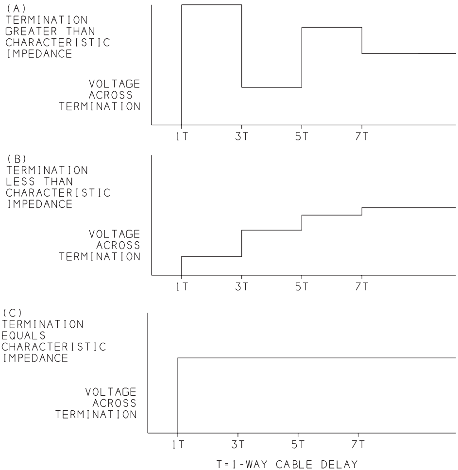
Figure 7-5: The initial voltages across a parallel termination vary depending on the difference between the termination and the line's characteristic impedance.
