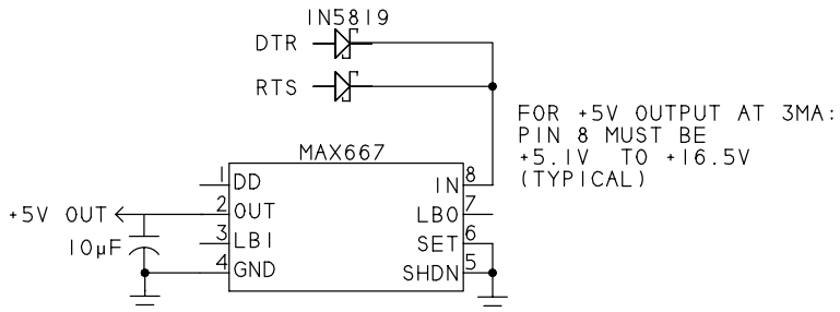
(B) REGULATED SUPPLY
