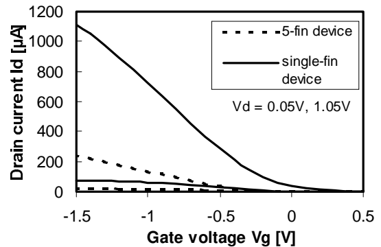
Figure 11: FinFET width can be adjusted quasi-continuously by the increment of a single fin (50-nm height)
