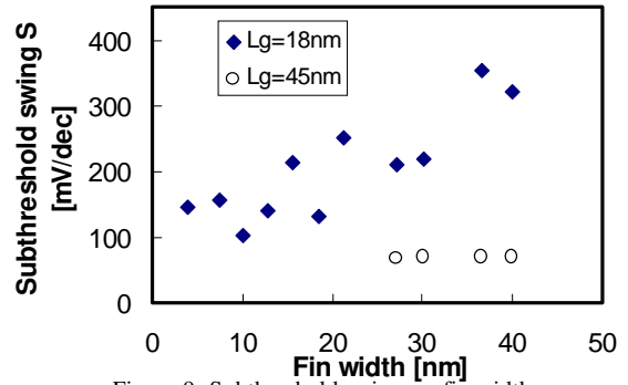
Figure 9: Subthreshold swing vs. fin width
