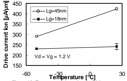
Figure 10: Temperature dependence of drive current.
