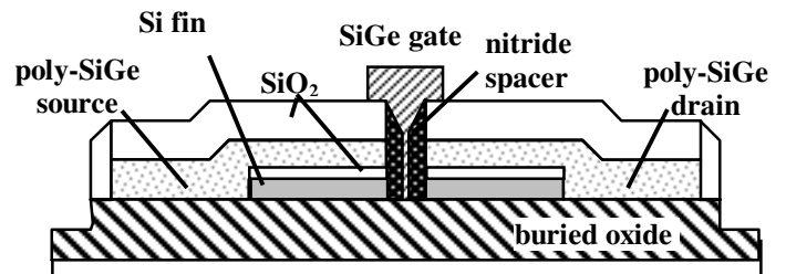
Figure 1: Schematic drawing of FinFET
