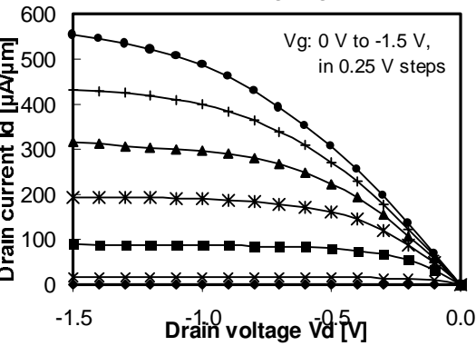
Figure 6: IV characteristics for 45-nm gate length and 30-nm thick Si body PMOS device
