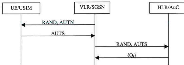
Figure 12: Resynchronisation mechanism
