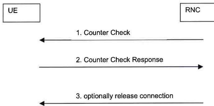
Figure 15a: RNC periodic local authentication procedure
