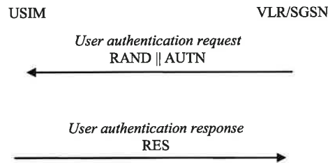
Figure 8: Successful UMTS Authentication and Key Agreement
