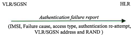
Figure 13: Reporting authentication failure from VLR/SGSN to HLR
