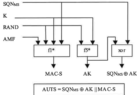
Figure 10: Construction of the parameter AUTS
