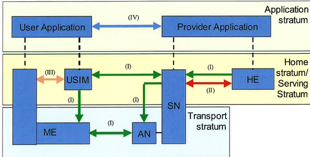
Figure 1: Overview of the security architecture
