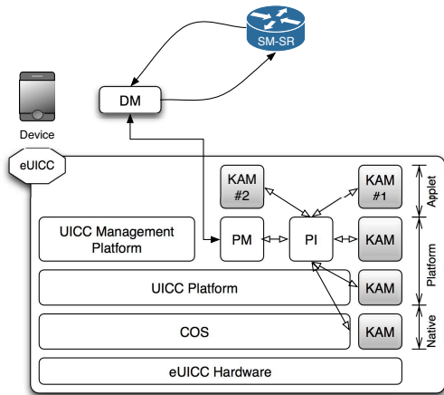
Fig. 5. Internal Architecture of eUICC
