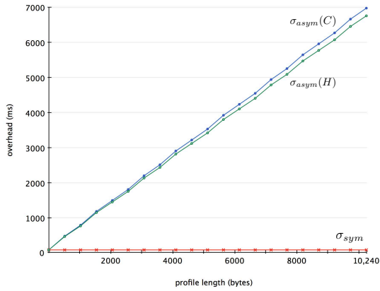
Fig. 6. Cryptography Performance of eUICC
