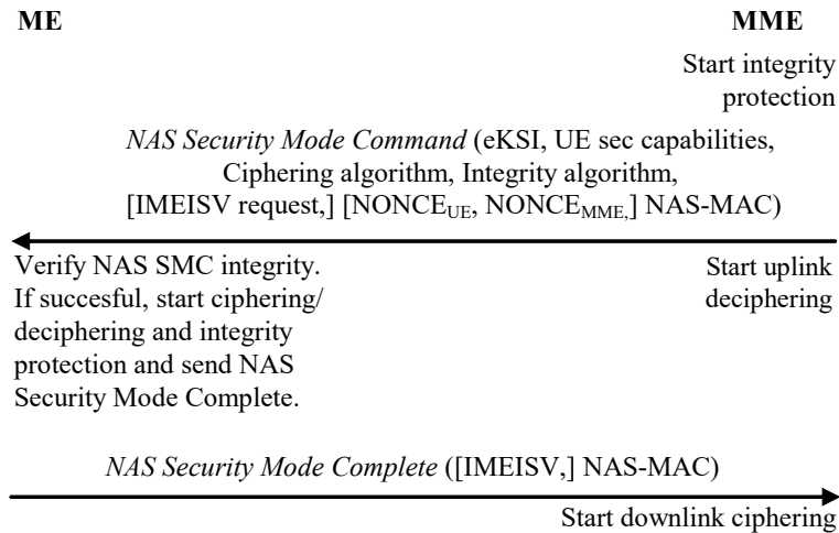
Figure 7.2.4.4-1: NAS security mode command procedure
