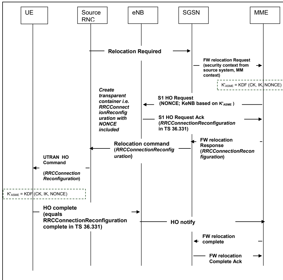
Figure 9.2.2.1-1: Handover from UTRAN to E-UTRAN
