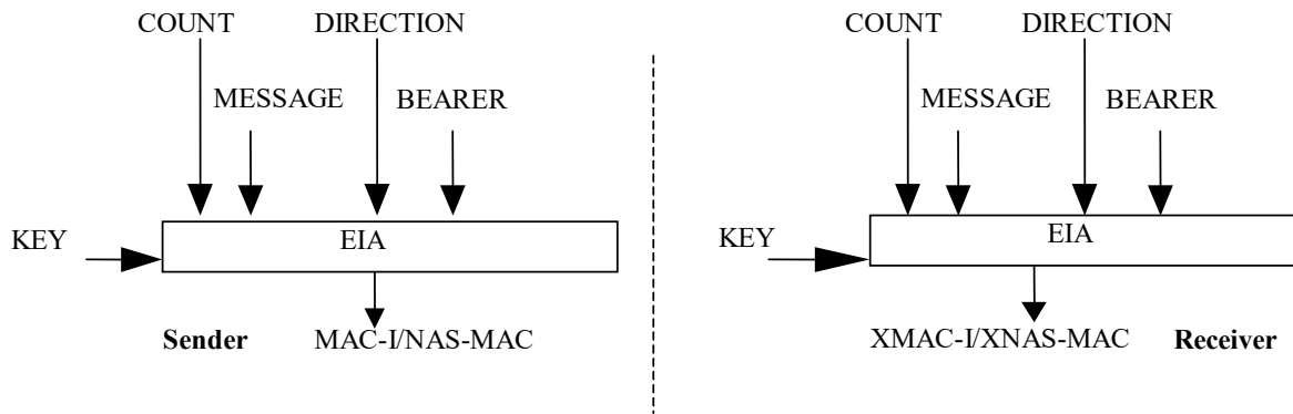
Figure B.2-1: Derivation of MAC-I/NAS-MAC (or XMAC-I/XNAS-MAC)
