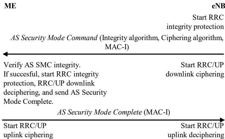
Figure 7.2.4.5-1: AS security setup
