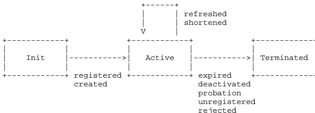
Figure 2: Contact State Machine
