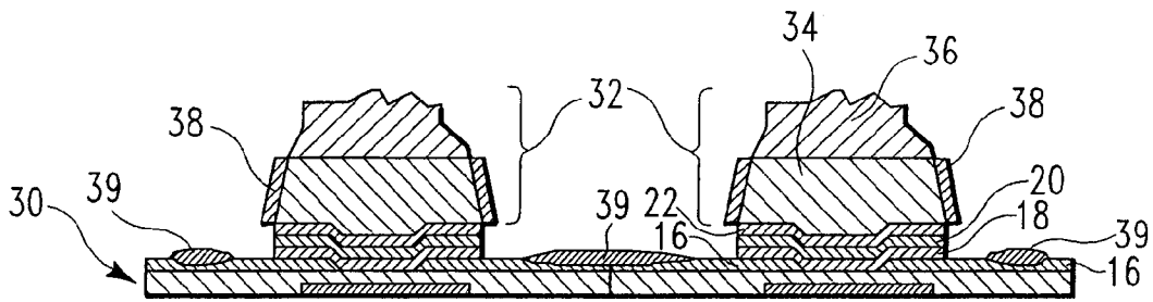
FIG. 3 PRIOR ART
