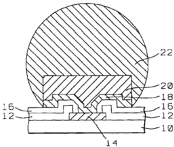
FIG. 4 - Prior Art
