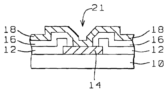
FIG. 2 - Prior Art
