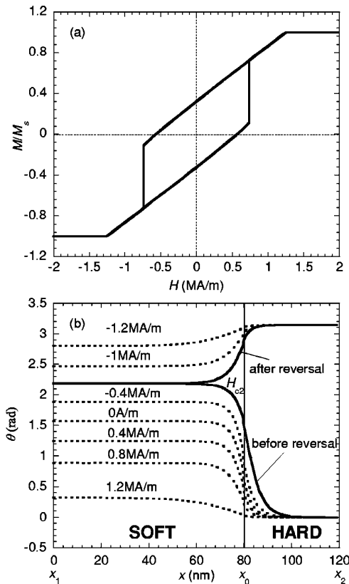
FIG. 3. (a) Major hysteresis loop for a FeRh/FePt bilayer with the parameters considered in Fig. 16, calculated assuming an interlayer coupling constant J_s with the same value of bulk coupling. (b) Behavior of the \vartheta(x) function in correspondence to different magnetic field values along the hysteresis loop.
