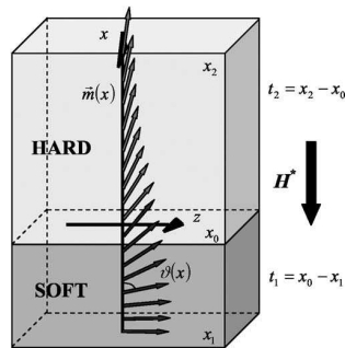
FIG. 1. Basic scheme for the one-dimensional continuum micromagnetic model of the hard/soft multilayer with anisotropy-axis perpendicular to the film plane.
