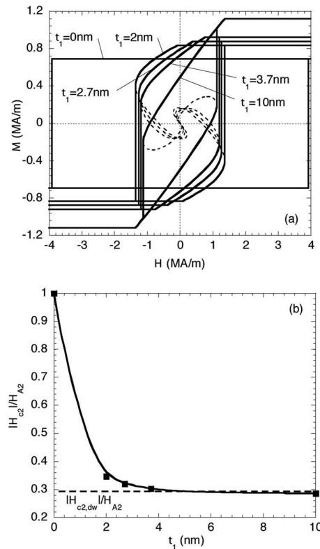
FIG. 4. (a) Calculated major hysteresis loops of the single layer FePt and of the Fe(t_1 \text{ nm})/FePt(10 \text{ nm}) bilayers (with the parameters reported in Sec. III): The dashed lines correspond to the unstable portion of the equilibrium curves. (b) The soft-thickness dependence of the reversal field H_{c2} [full line: t_2 fixed to 10 nm; dashed line: (t_1, t_2) \rightarrow \infty ], normalized to the hard-phase anisotropy field H_{A2} = 2L_2 / (\mu_0 M_2) .
