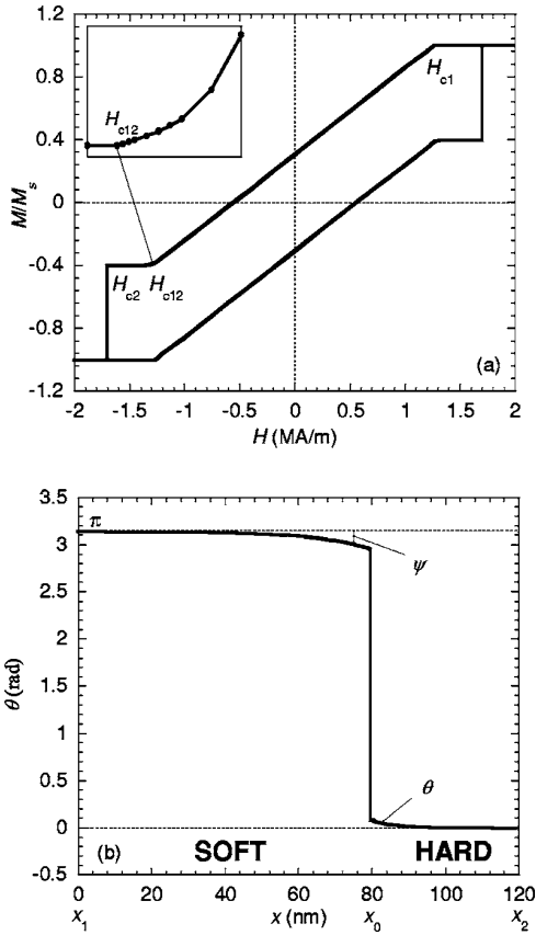
FIG. 7. (a) Major hysteresis loop for a FeRh/FePt bilayer with the parameters considered in Fig. 16, calculated assuming an inter-layer exchange constant J_s = 0.02 \times J_{s\text{-bulk}} . Inset: enlarged-scale portion of the loop in the region close to the critical field H_{c12} . (b) Behavior of the \vartheta(x) and the \psi(x) = \pi - \vartheta(x) functions, corresponding to the magnetic field value H = -H^* = -1.34 MA/m (which is slightly below the critical field H_{c12} ).
