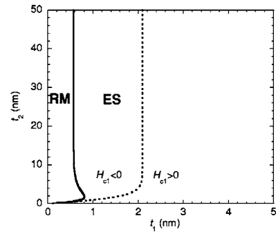
FIG. 2. Magnetic phase diagram in the plane of layer thicknesses t_1 (soft) and t_2 (hard) for a Fe/FePt bilayer with perpendicular anisotropy and the parameters reported in Sec. III. The figure reports the critical \chi_c line ( \chi_c \rightarrow \infty , full line) together with the isofield line corresponding to H_{c1}=0 (dashed line). RM =rigid magnet; ES =exchange-spring magnet.
