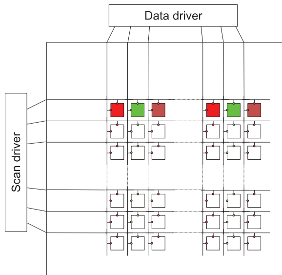
Figure 4.19 Matrix driving of a passive-type OLED display.
