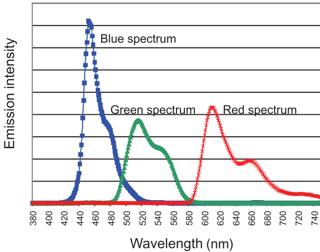
Figure 4.11 Example of emission spectrum of RGB (red + green + blue) subpixels.
