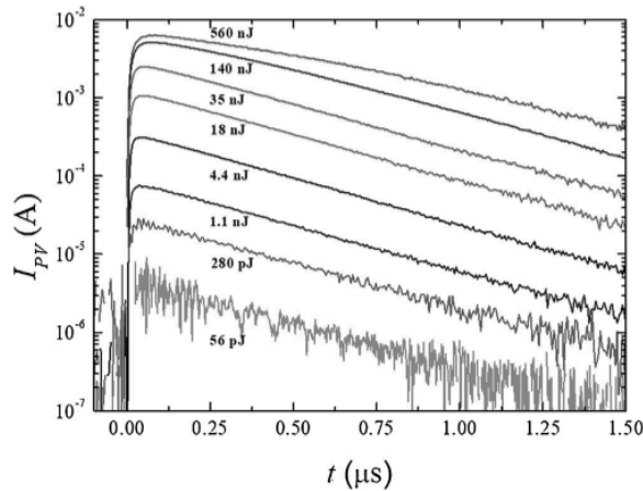
Fig. 2. Photocurrent vs. time collected in the photovoltaic mode at different energies of the nanosecond light pulse.
