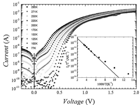
Fig. 5. Current-voltage characteristics for the SWCNT/Si junctions in dark conditions at different temperature. Inset: saturation current I_0 vs. temperature for the same sample of the main panel. The values of I_0 are obtained by linear extrapolation to zero voltage of the low current data ( V < 100 mV) of the main panel. The straight line is a fit to the data which well approximates the experimental points in the range T = 300 K–140 K.
