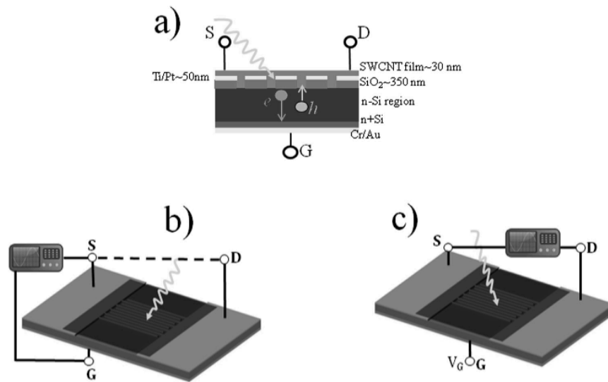
Fig. 1. (a) Schematic section of the SWCNT/Si photodetector with the photocharges drifted towards the opposite electrodes by the interface built-in potential; (b) three dimensional view of the photodetector with the terminals connected for photovoltaic and (c) photoconductive measurements.
