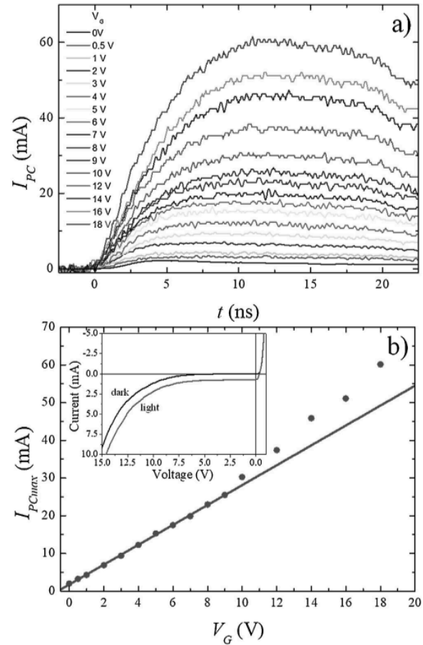
Fig. 3. (a) Photocurrent vs. time collected in the photoconductive mode at different values of the gate voltage V_G ; (b) maximum of the curves shown in a) as a function of V_G . The straight line is a fit to the data in the range V_G = 0 –9 V. Inset: Current voltage characteristics of the same device measured in the photovoltaic mode under dark and light conditions.
