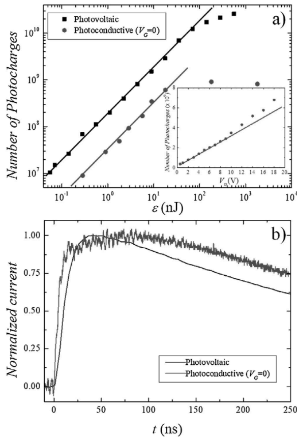
Fig. 4. (a) Number of photocharges collected in photovoltaic (black squares) and photoconductive (red circles) mode as a function of the light pulse energy. The lines are linear fit to the data for \epsilon < 30 nJ; Inset: number of photocharges collected in photoconductive mode as a function of the gate voltage V_G . (b) normalized photocurrent with respect to its maximum value as a function of the time in the photovoltaic (black lower curve) and photoconductive (red upper curve) mode. (For interpretation of the references to colour in this figure legend, the reader is referred to the web version of this article).
