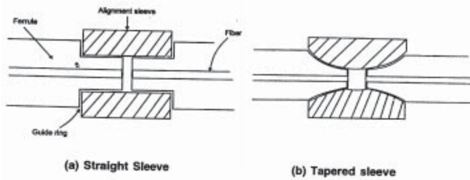
Figure 7. Connectors using butt-joint alignment designs.
