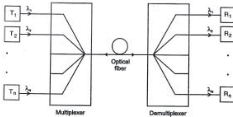
Figure 9. Multichannel point-to-point fiber link. T - transmitter; R - receiver.
