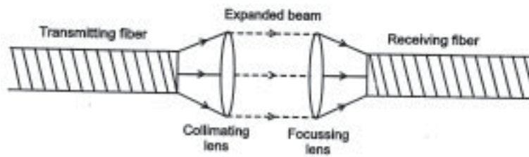
Figure 8. Expanded beam connector.
