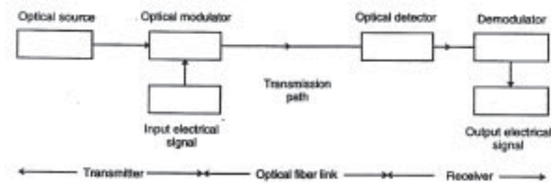
Figure 2. Basic analog optical fiber communication system.
