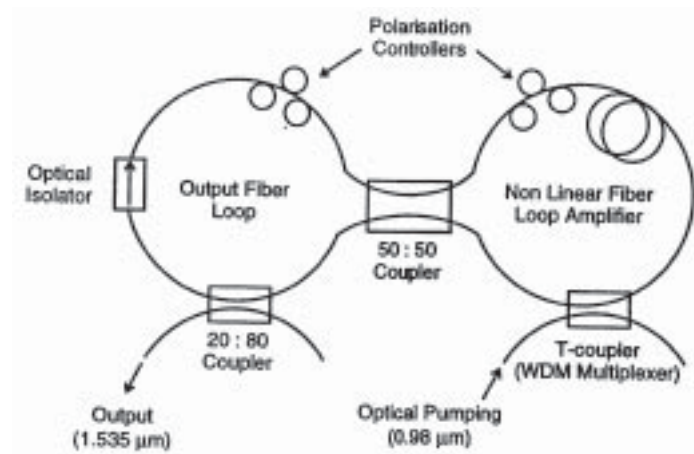
Figure 11. Figure – 8 laser.
