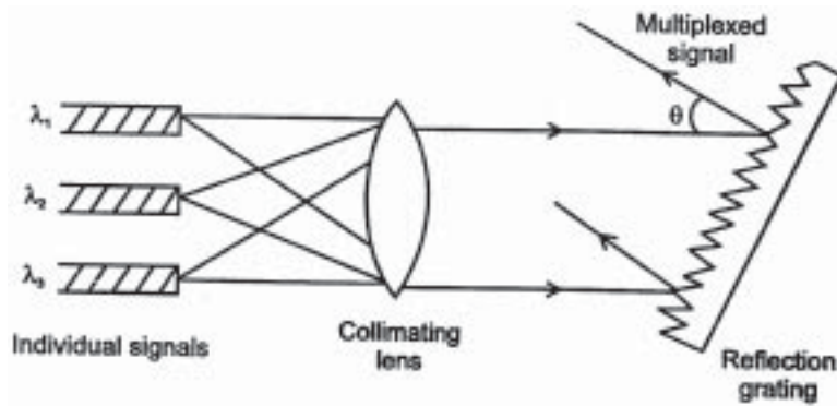
Figure 10. Grating multiplexer.
