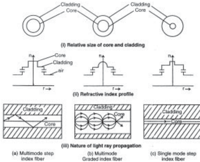
Figure 1. Different types of fibers.
