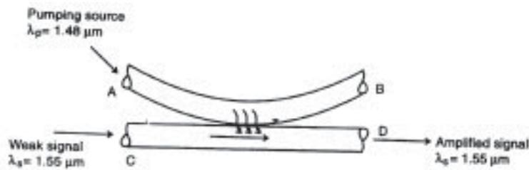
Figure 4. Optical fiber laser amplifier.
