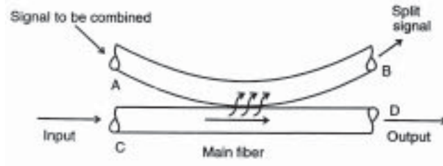
Figure 6. Four port coupler.
