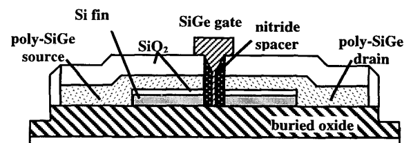
Figure 1: Schematic drawing of FinFET
