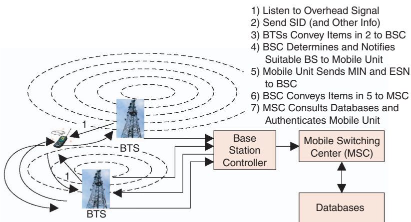
Fig. 2 Major steps in a cell phone connecting to a mobile/cellular network
