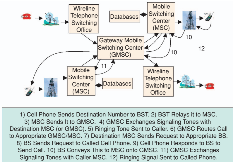
Fig. 3 Major steps indicating how a call goes through a mobile/cellular network
