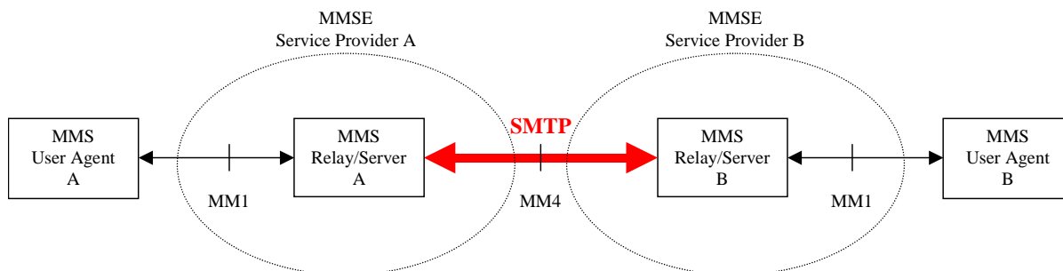
Figure 8: Interworking of different MMSEs[2]
