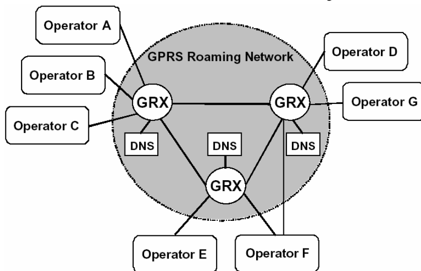
Figure 10: GPRS Roaming network architecture: [4]
