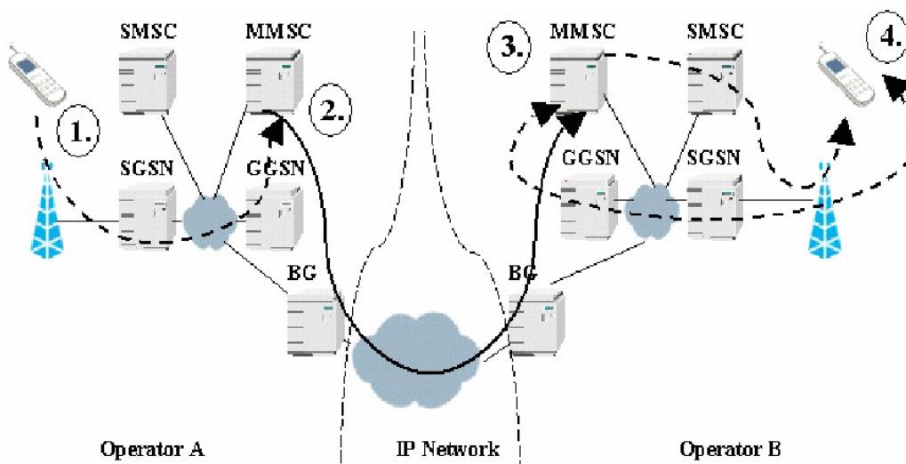
Figure 9: Interworking of different MMSEs[5]
