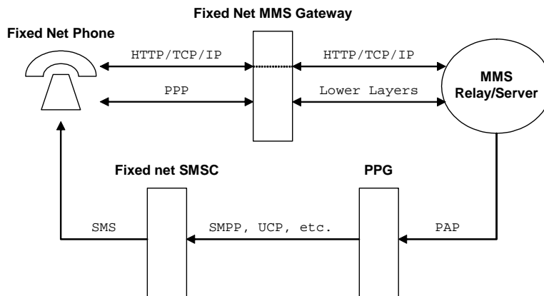
Figure 12: General MM1 gateway structure for fixed networks[3]
