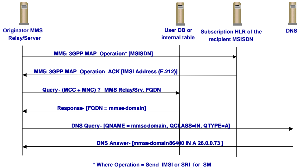
Figure 11: Message flow of the recipient MSISDN address resolution based on IMSI [2]
