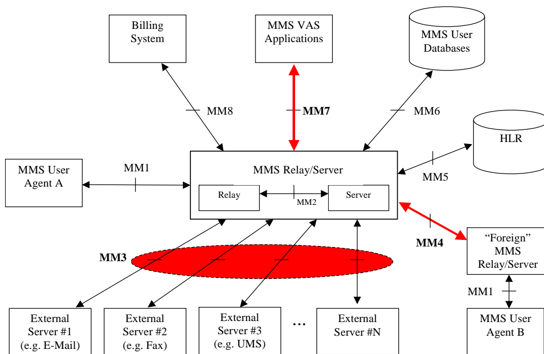
Figure 7: MMS Reference Architecture [2]
