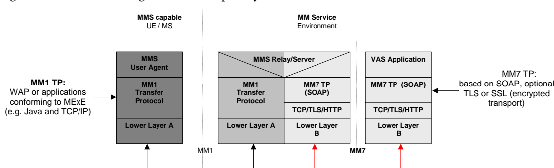
Figure 13: MM7 Service Environment, mapping to MM1
