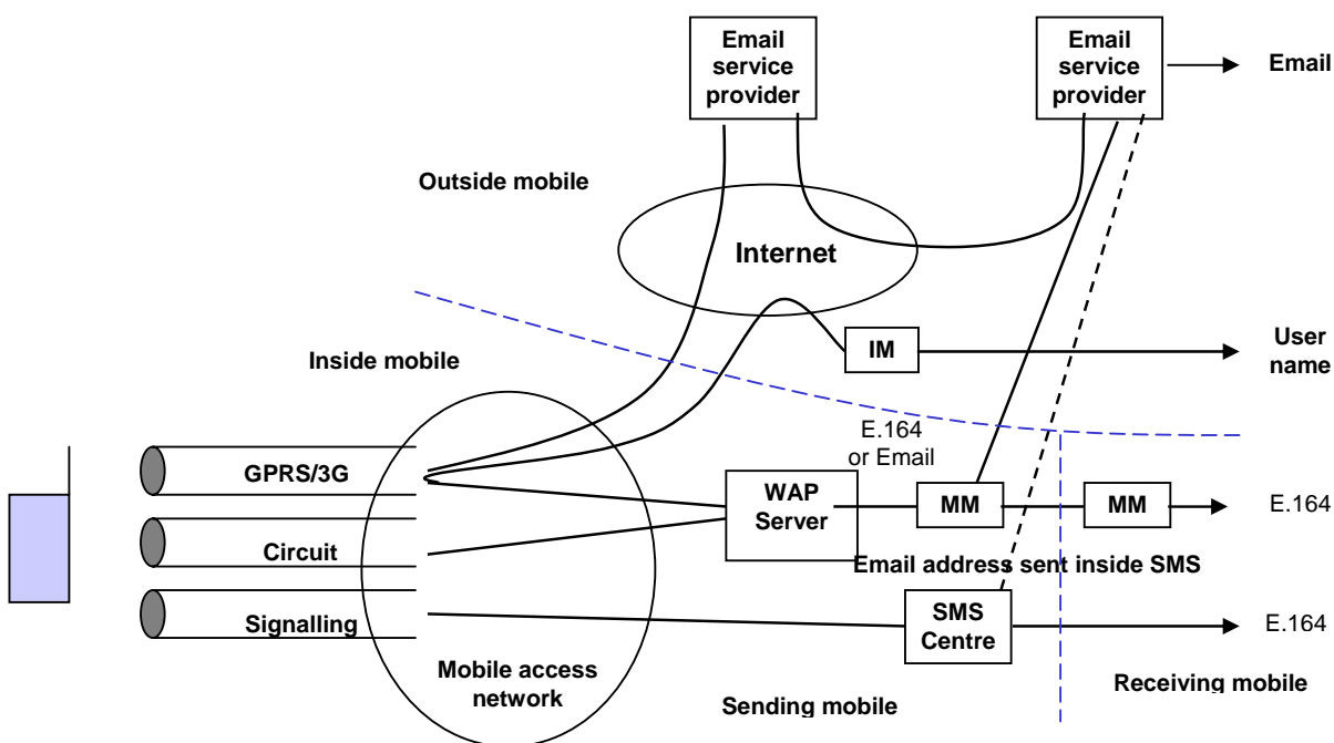
Figure 3: Principle of MMS communications
