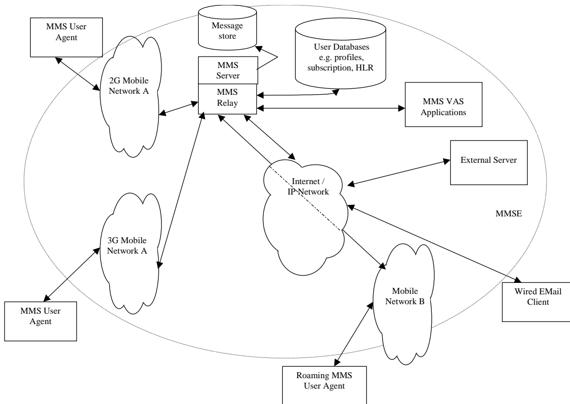
Figure 6: MMS Architectural Elements[2]
