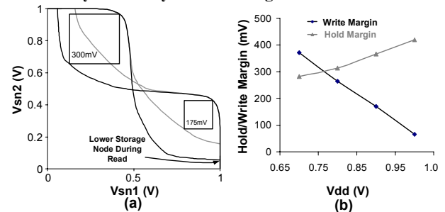
Figure 8. (a) Read SNM plot for a FinFET 6-T cell with feedback. (b) Impact of cell supply on write margin and standby SNM. Approximately 300mV of write margin and standby SNM can be achieved with a cell bias of 0.8V.
