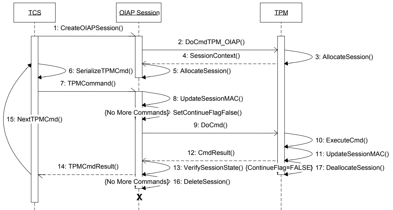
Figure 4:1 - OLAP Sequence
