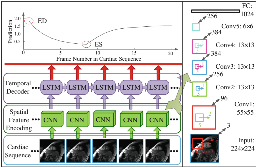
Fig. 2. An overview of the proposed framework, temporal regression network (TempReg-Net). Note that only convolutional layers are shown and Conv1 and Conv2 and Conv5 layers are followed by Pooling layers of size 3 \times 3 and stride 2.
