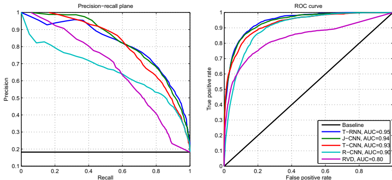
Fig. 5. The PR plane and ROC curves of different methods on FASP detection.
