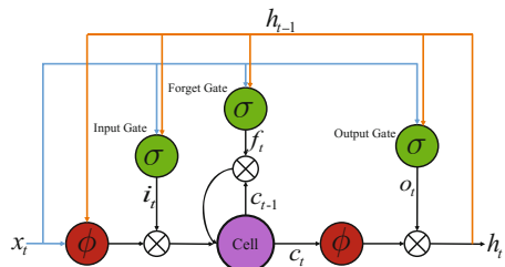
Fig. 3. LSTM model
