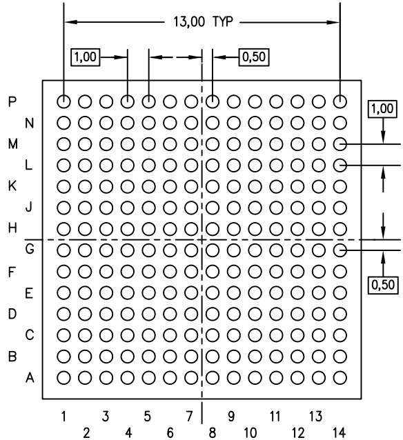
Plastic Ball Grid Array 196 Balls Bottom View
