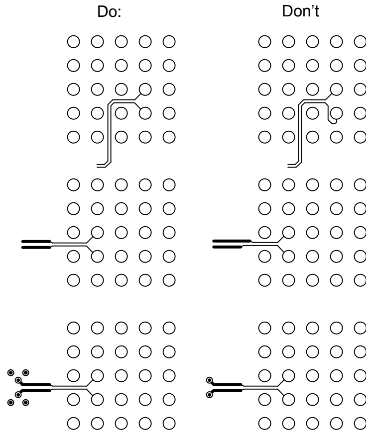
Figure 10. Layout Guidelines
