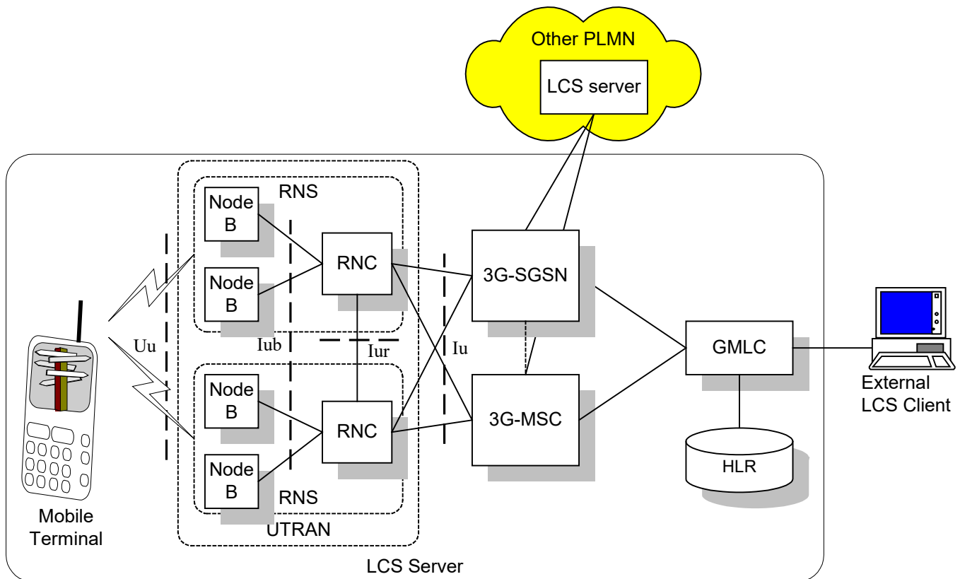
Figure 6.1, General arrangement of LCS in UMTS
