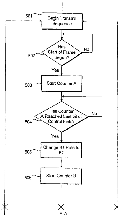
METHOD OF SWITCHING FROM F1 TO F2 ETC FLOW CHART
