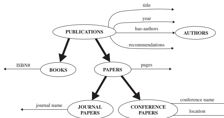
Figure 12 Subclasses, superclasses, and attribute inheritance.
