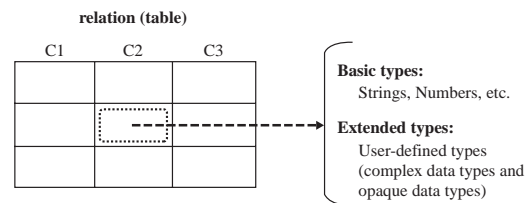
Figure 14 Extending domain types in a relation.
