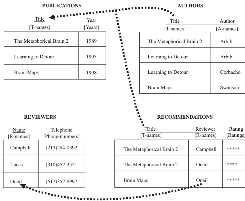
Figure 3 Example relational database.
