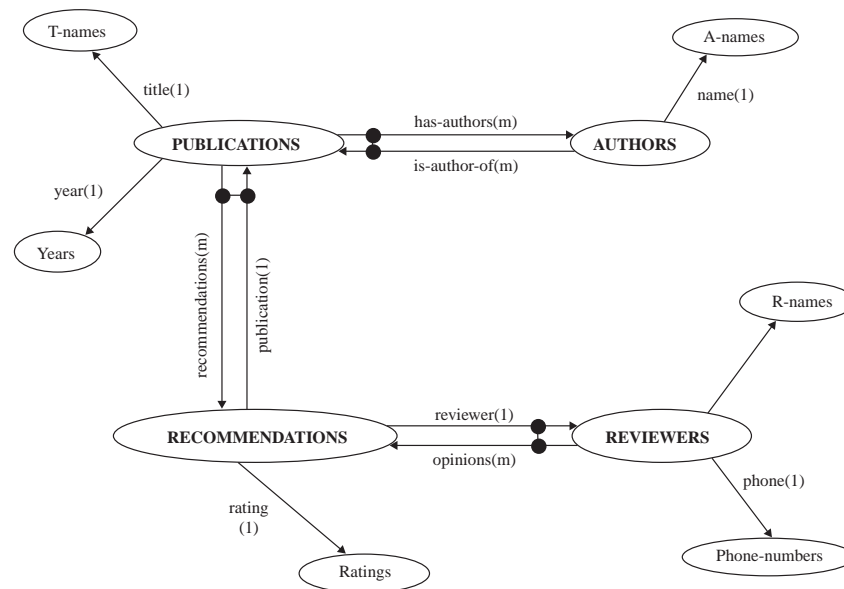
Figure 10 Classes and attributes.
