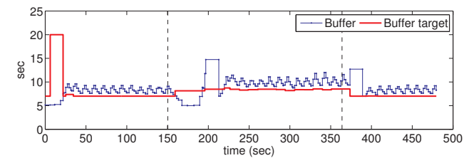
(c) Receiver buffer length and target buffer length
