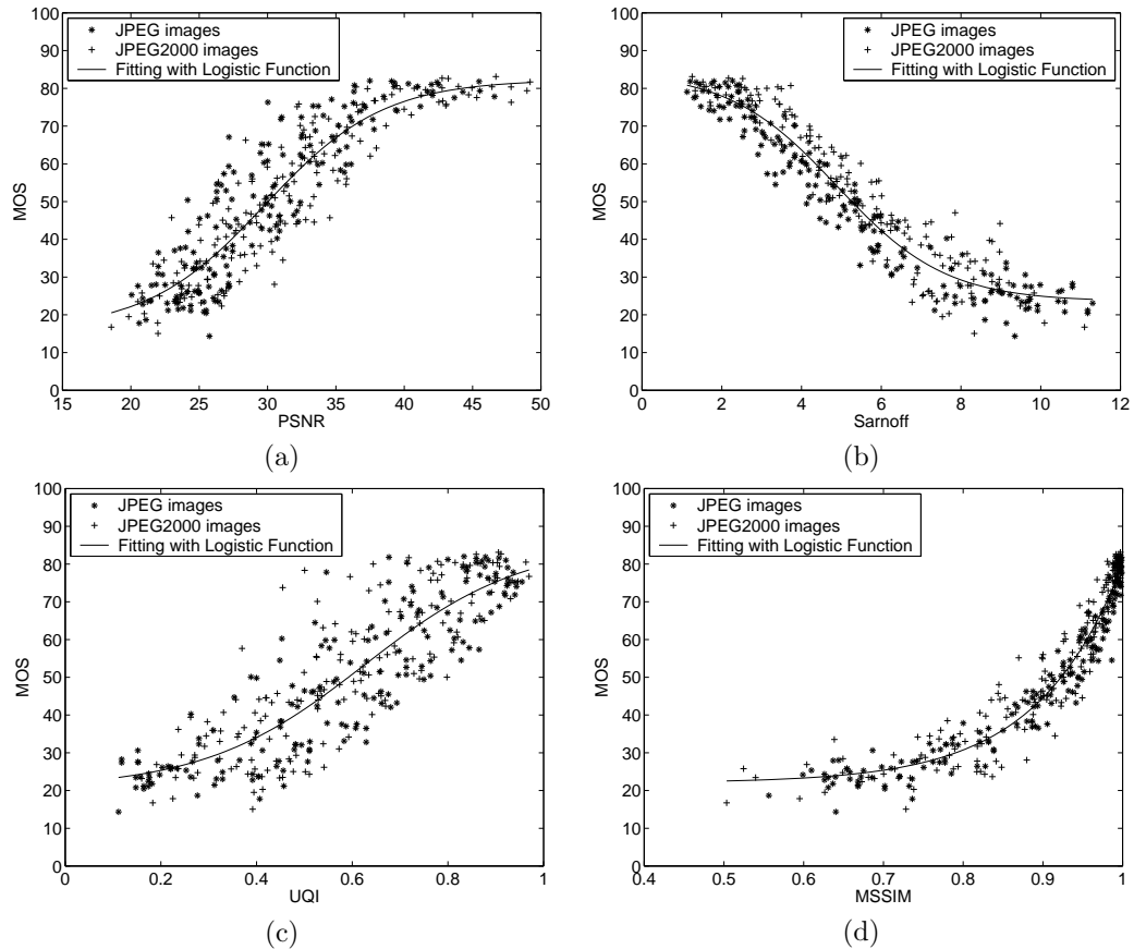
Fig. 8. Scatter plots of subjective mean opinion score (MOS) versus model prediction. Each sample point represents one test image. (a) PSNR; (b) Sarnoff model [56]; (c) UQI [7] (equivalent to MSSIM with square window and K_1 = K_2 = 0 ); (d) MSSIM (Gaussian window, K_1 = 0.01, K_2 = 0.03 ).
