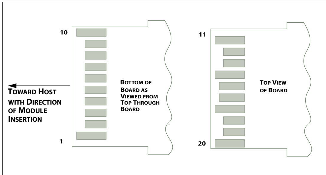
Figure 2 SFP+ module contact assignment
