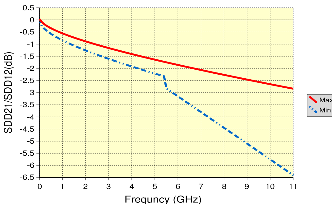
Figure 42 Mated MCB-HCB Differential Through Response Limits
