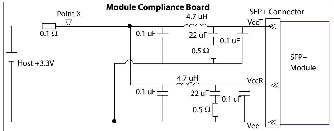
Figure 56 Module Compliance Board Power Supply Filters
