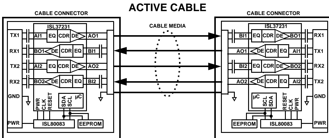
FIGURE 1. TYPICAL APPLICATION
