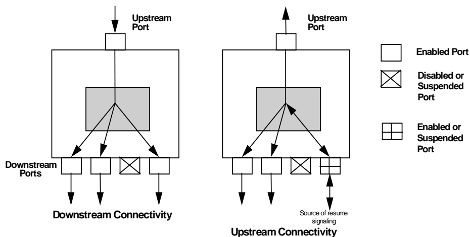
Figure 11-3. Resume Connectivity
