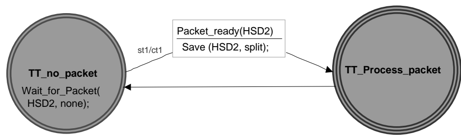
Figure 11-38. Transaction Translator
