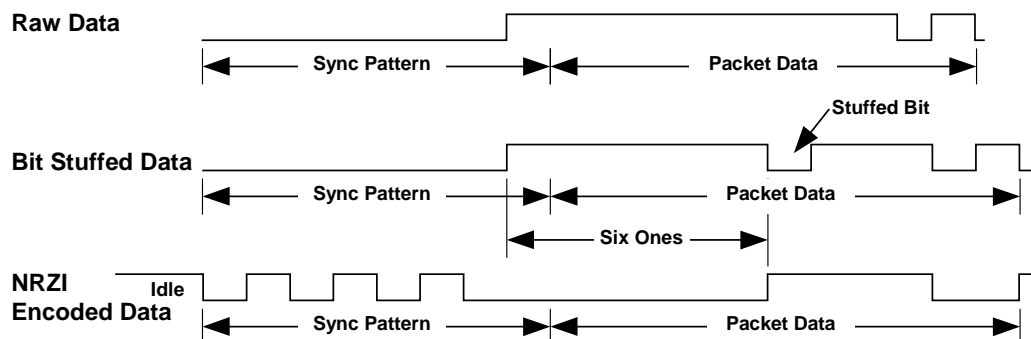
Figure 7-32. Bit Stuffing
