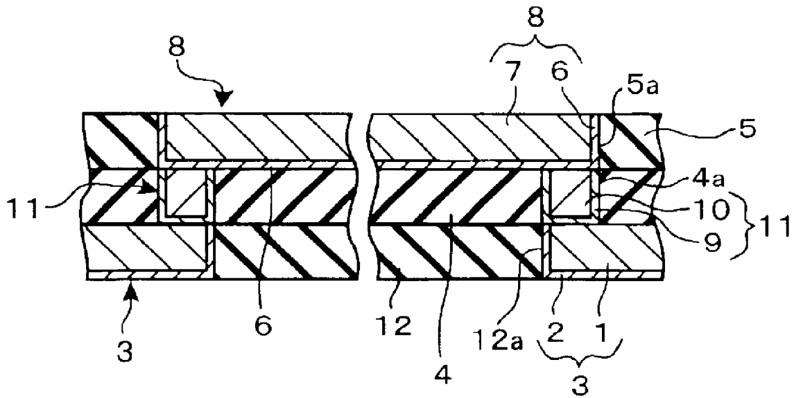
FIG. 19 (Prior Art)
