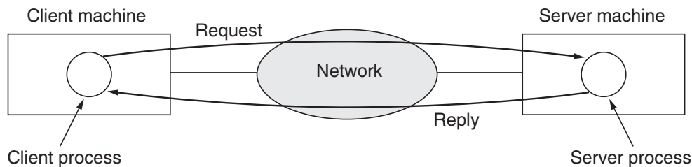
Figure 1-2. The client-server model involves requests and replies.
