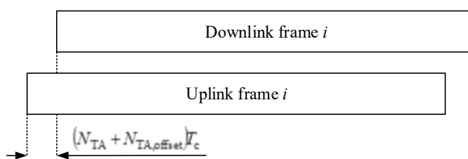
Figure 4.3.1-1: Uplink-downlink timing relation.
