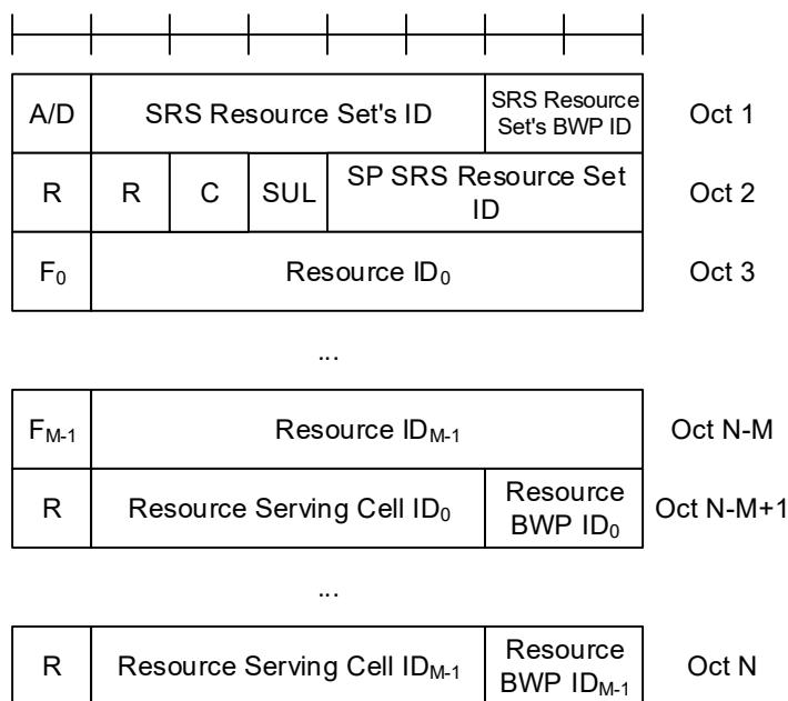
Figure 6.1.3.17-1: SP SRS Activation/Deactivation MAC CE
