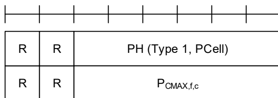
Figure 6.1.3.8-1: Single Entry PHR MAC CE
