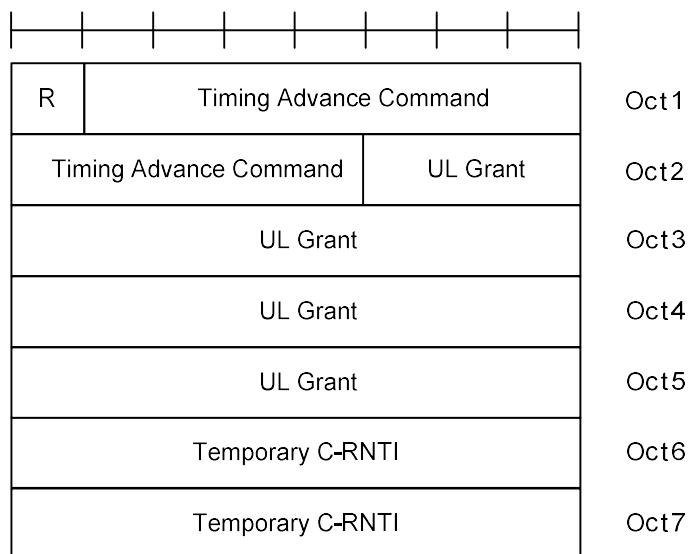
Figure 6.2.3-1: MAC RAR
