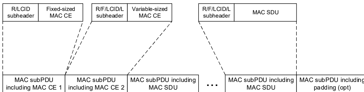
Figure 6.1.2-4: Example of a DL MAC PDU
