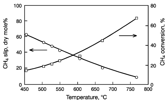
Fig. 1. FT diesel conversion over RKNR ( H_2O/C = 3.7 , 25 bar).
