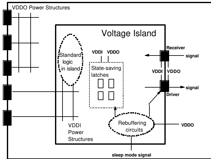
Fig.5. Voltage Island Powering and Switching Control
