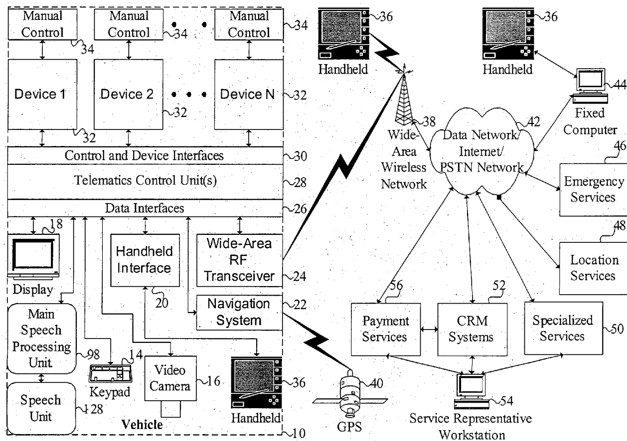
Figure 2. Second Embodiment System Block Diagram
