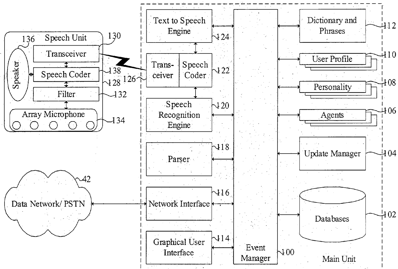
Figure 5. Speech Processing System Block Diagram
