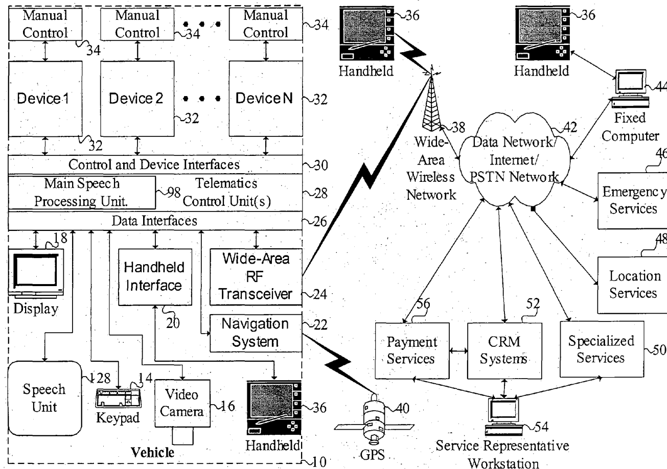
Figure 1. First Embodiment System Block Diagram
