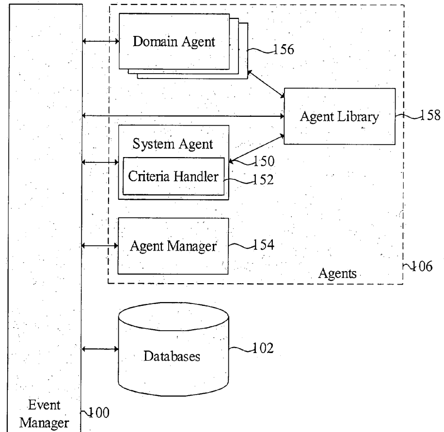
Figure 6. Agent Architecture
